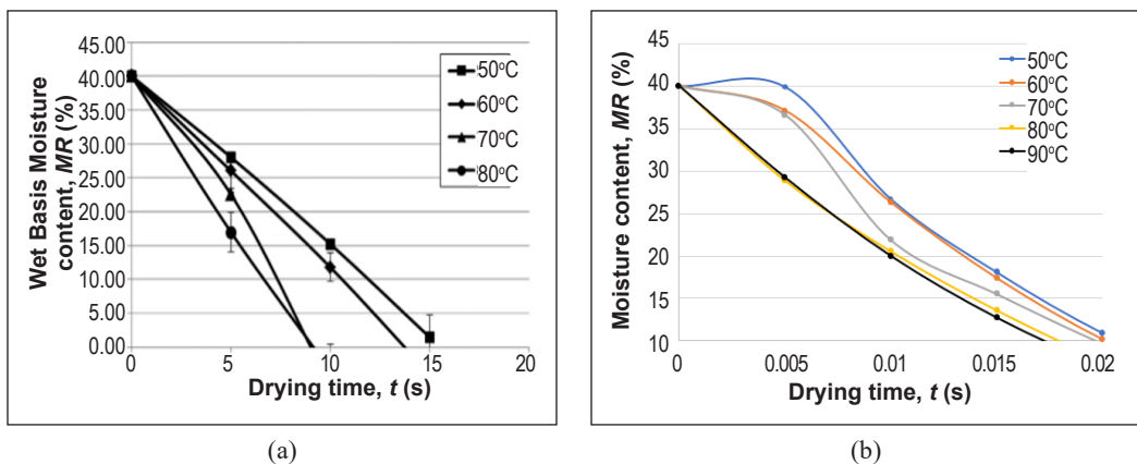
Figure 10. Moisture content against drying time of: (a) Previous studies; and (b) this CFD simulation
