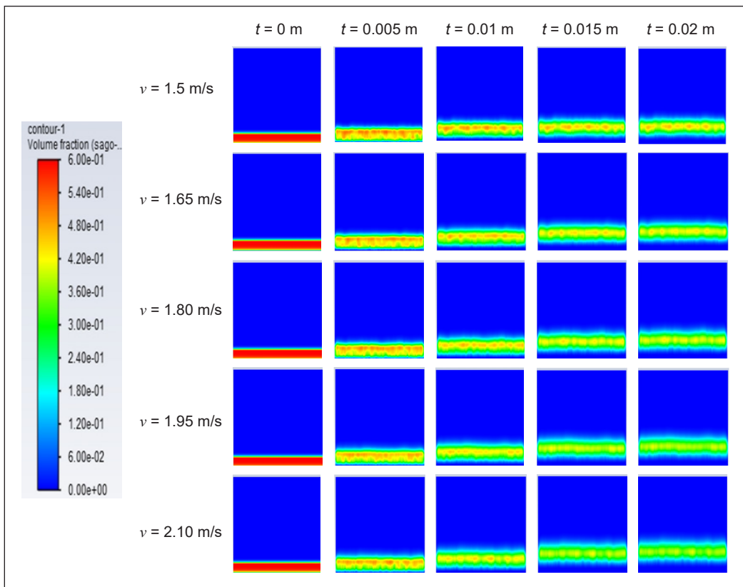
Figure 6. Contour of sago waste volume fraction at air velocity, v_i=1.5\text{-}2.1 m/s
