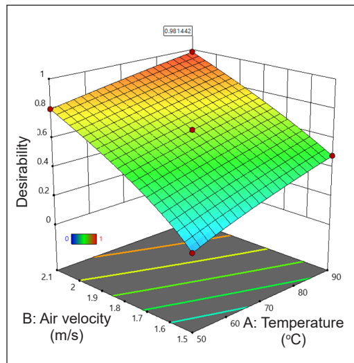
Figure 9. Desirability surface plot for sago bagasse diameter 2000 µm
