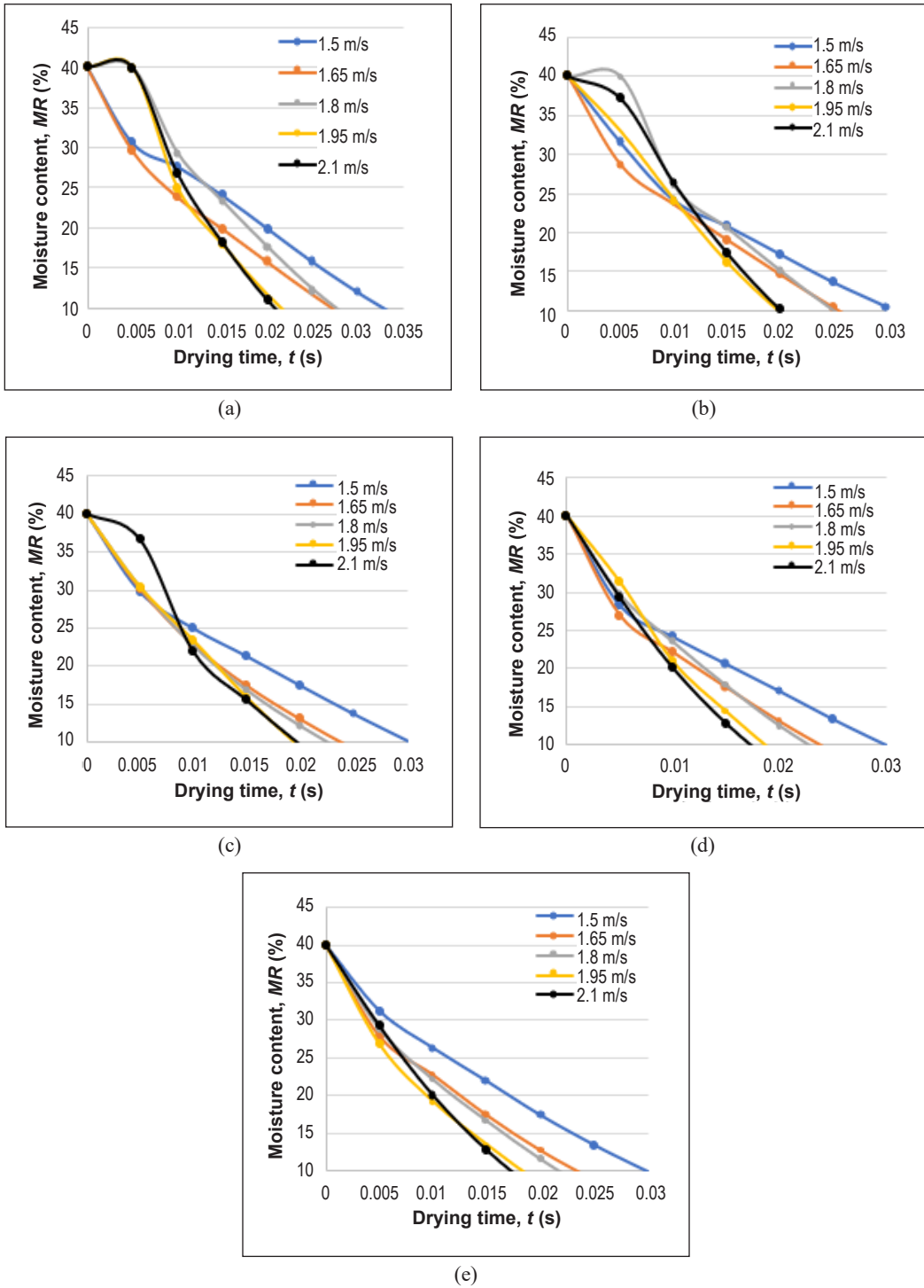
Figure 7. Moisture content against drying time at the diameter of 2000\ \mu\text{m} with different air velocity temperatures and temperatures: (a) T=50^{\circ}\text{C} ; (b) T=60^{\circ}\text{C} ; (c) T=70^{\circ}\text{C} ; (d) T=80^{\circ}\text{C} ; and (e) T=90^{\circ}\text{C}
