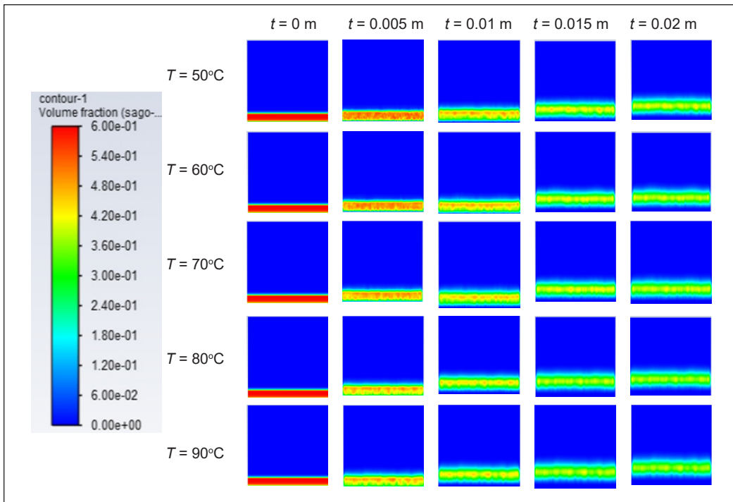
Figure 4. The contour of sago waste volume fraction at various temperatures: 50–90°C
